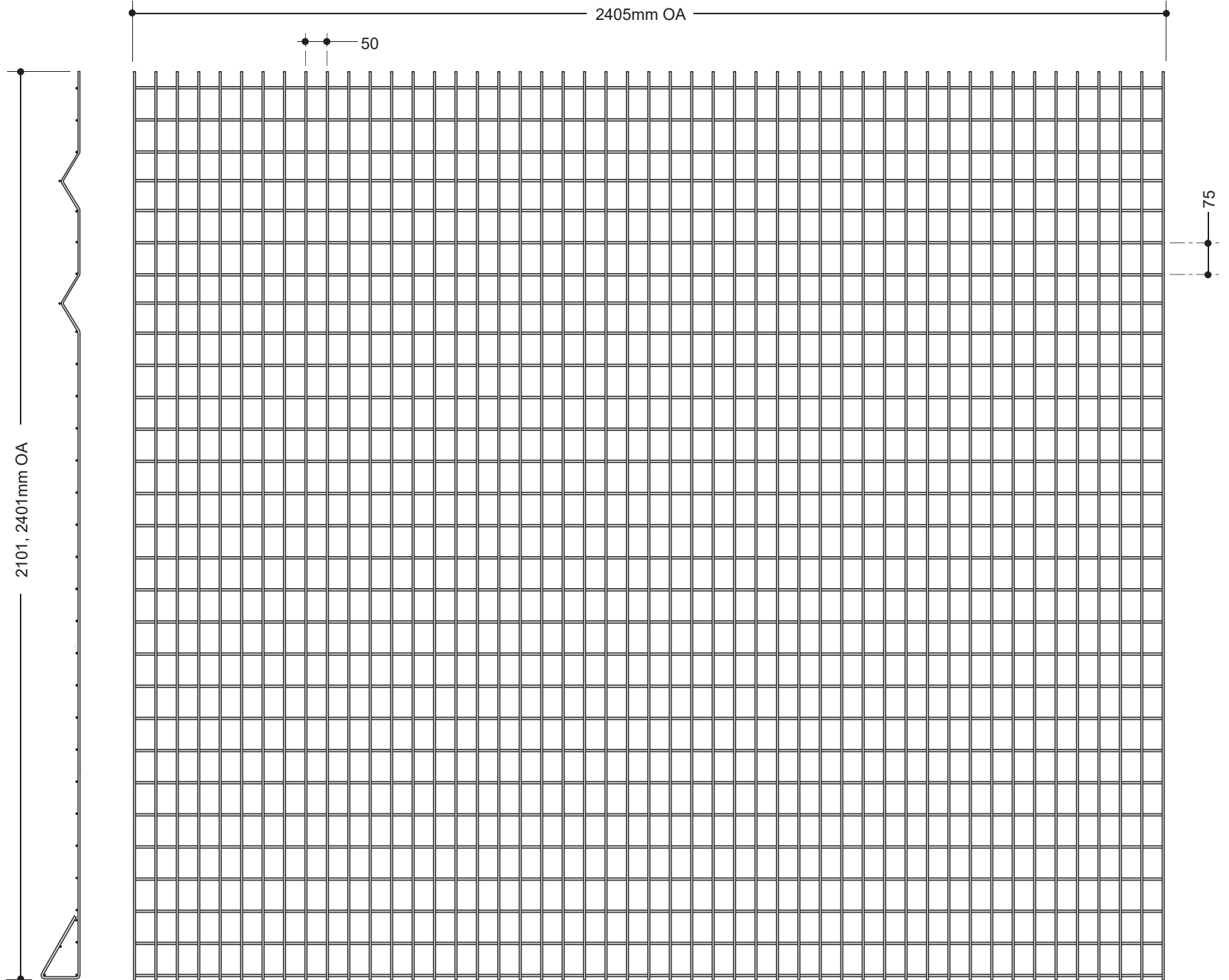
BOULEVARD SECURITY - WELDED MESH PANELS
