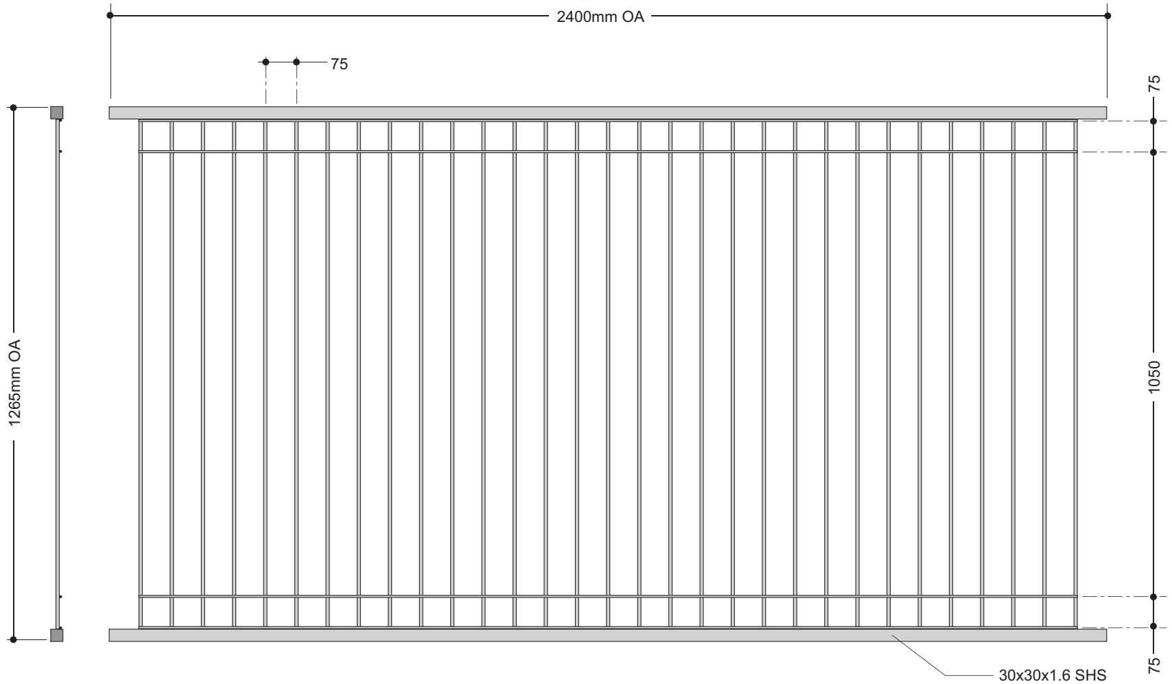
WILLOW COMMERCIAL - WELDED MESH PANEL
