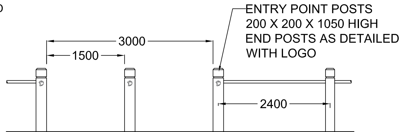
INSTALLATION ELEVATION
