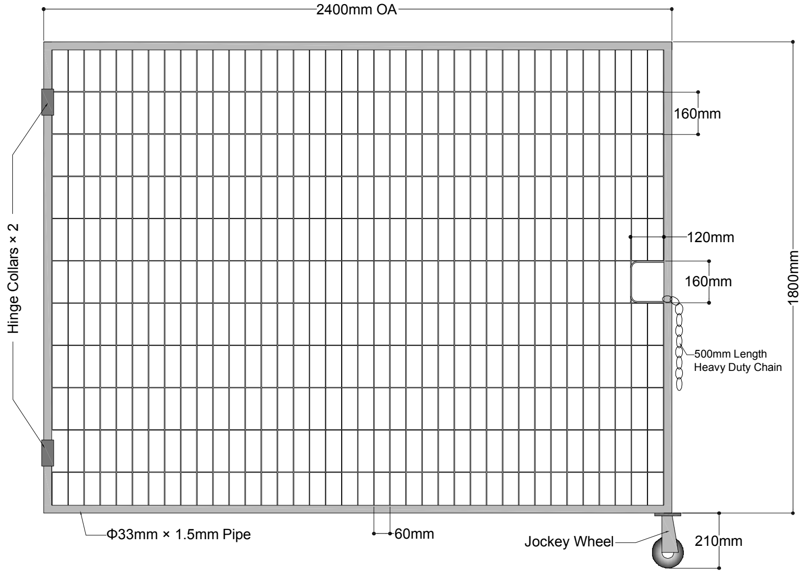
TEMPORARY FENCE GATE
